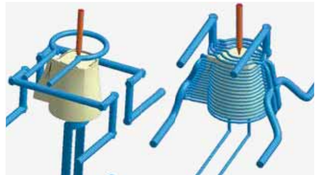
Conventional cooling
